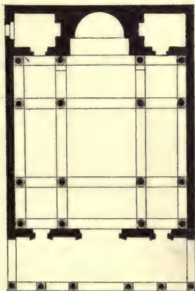
Fig. 24.—Plan of Church at Musmieh (IIInd and IIIrd Centuries).
